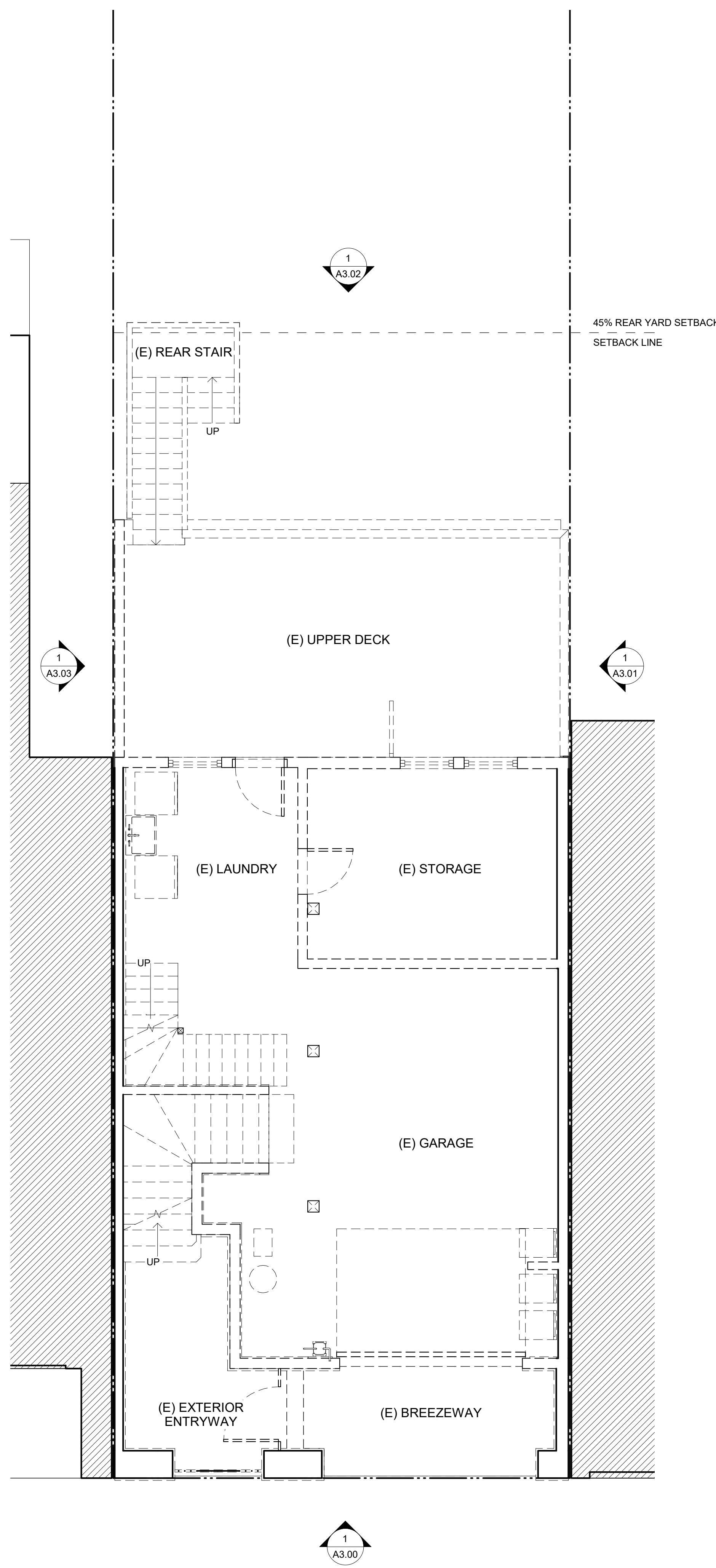
2 GROUND FLOOR - EXISTING / DEMO PLAN 1/4" = 1'-0"
