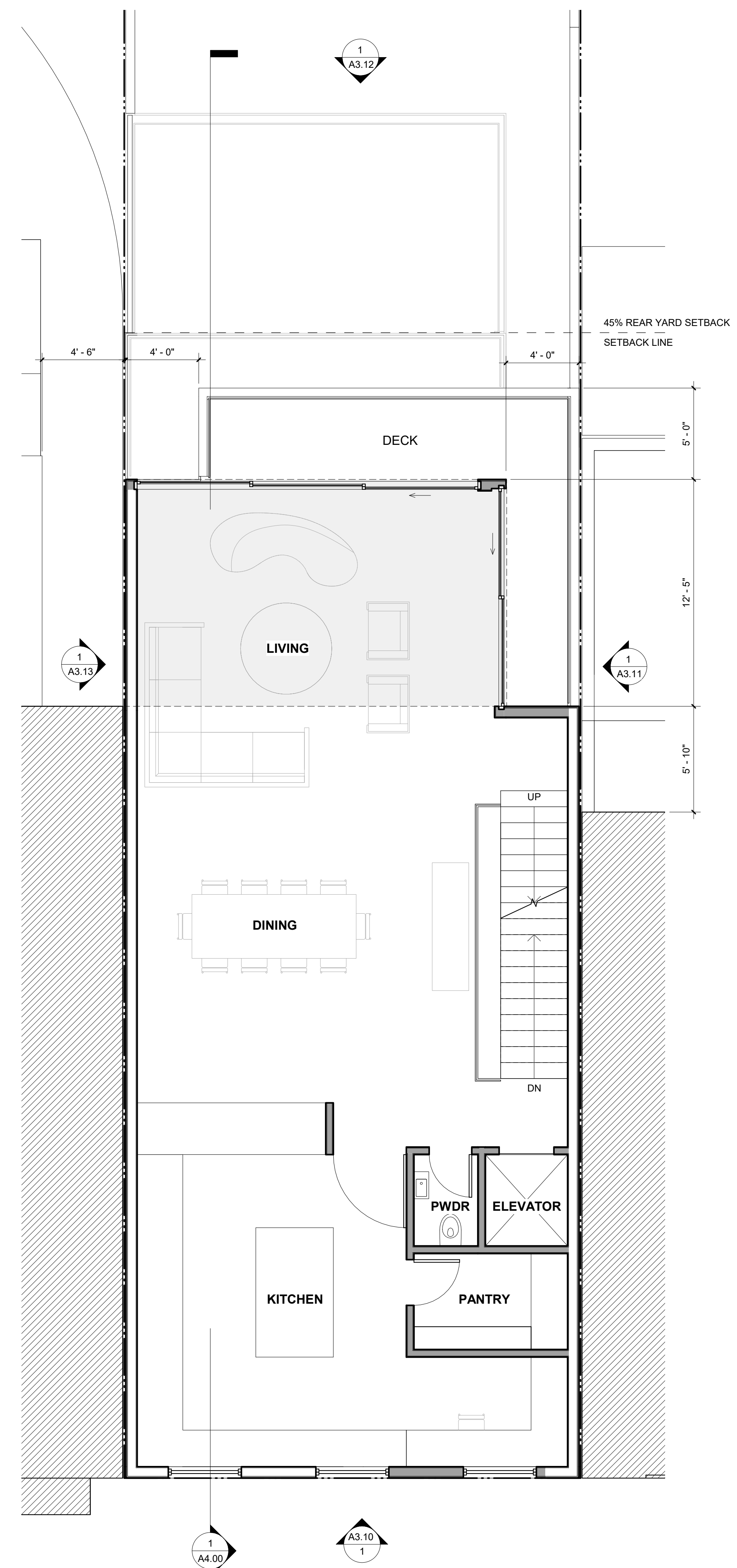
1 LEVEL 2 - PROPOSED PLAN 1/4" = 1'-0"
