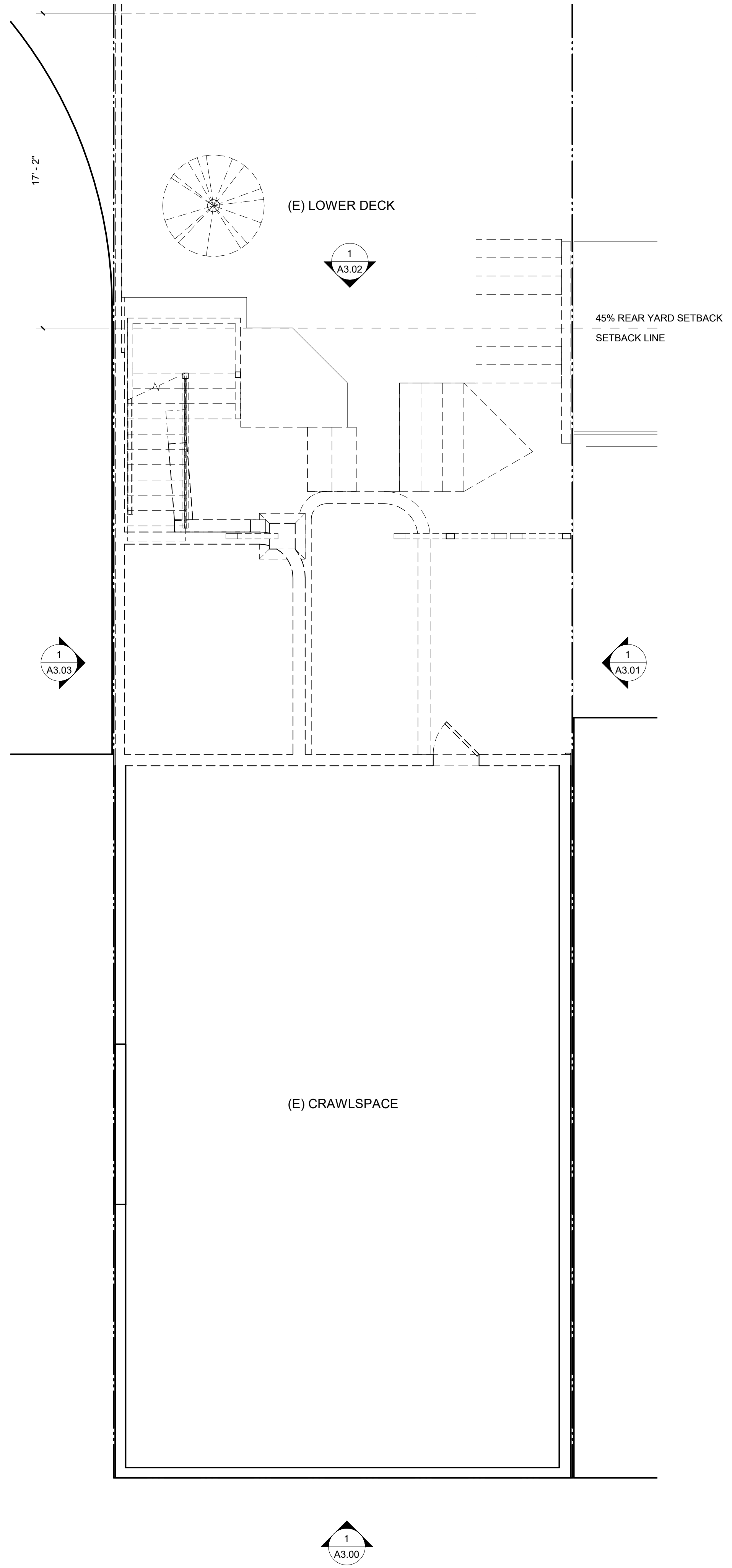
2 BASEMENT - DEMO PLAN 1/4" = 1'-0"
