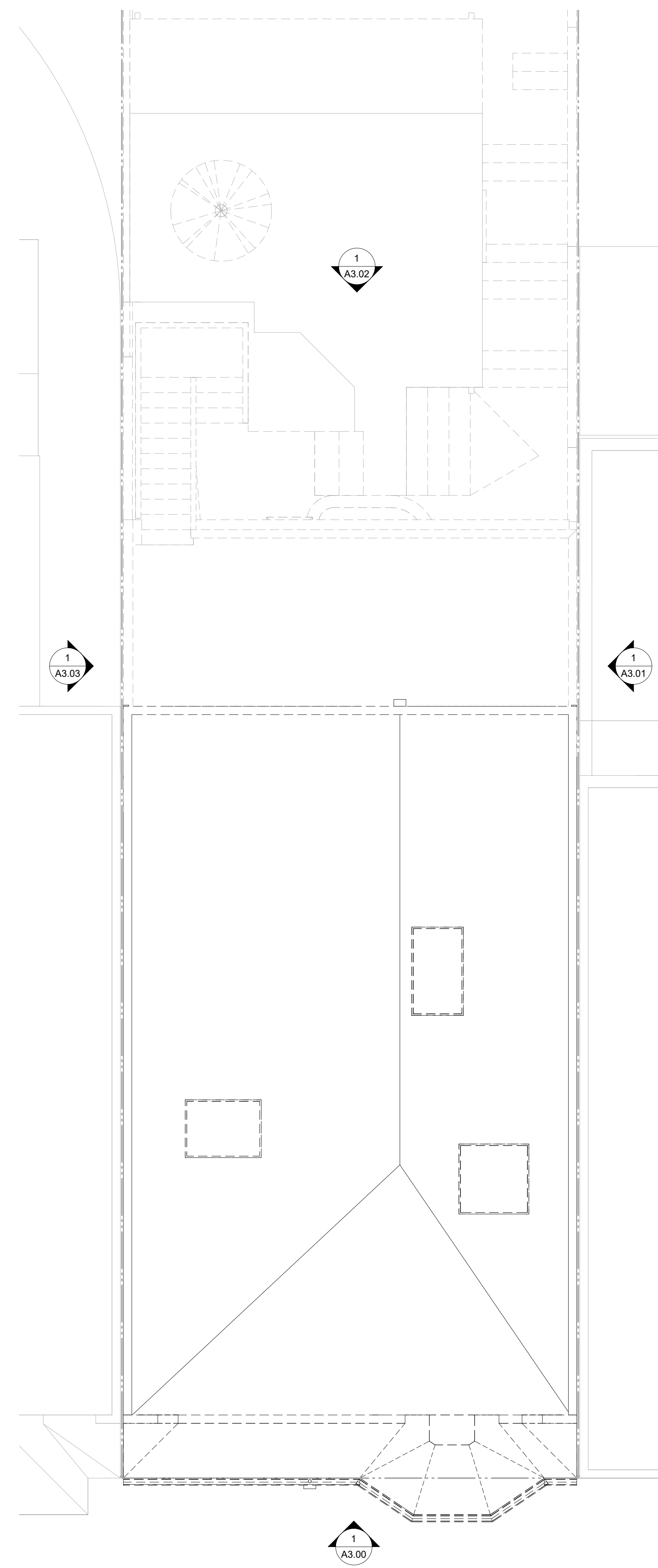
2 ROOF PLAN - EXISTING / DEMO PLAN 1/4" = 1'-0"
