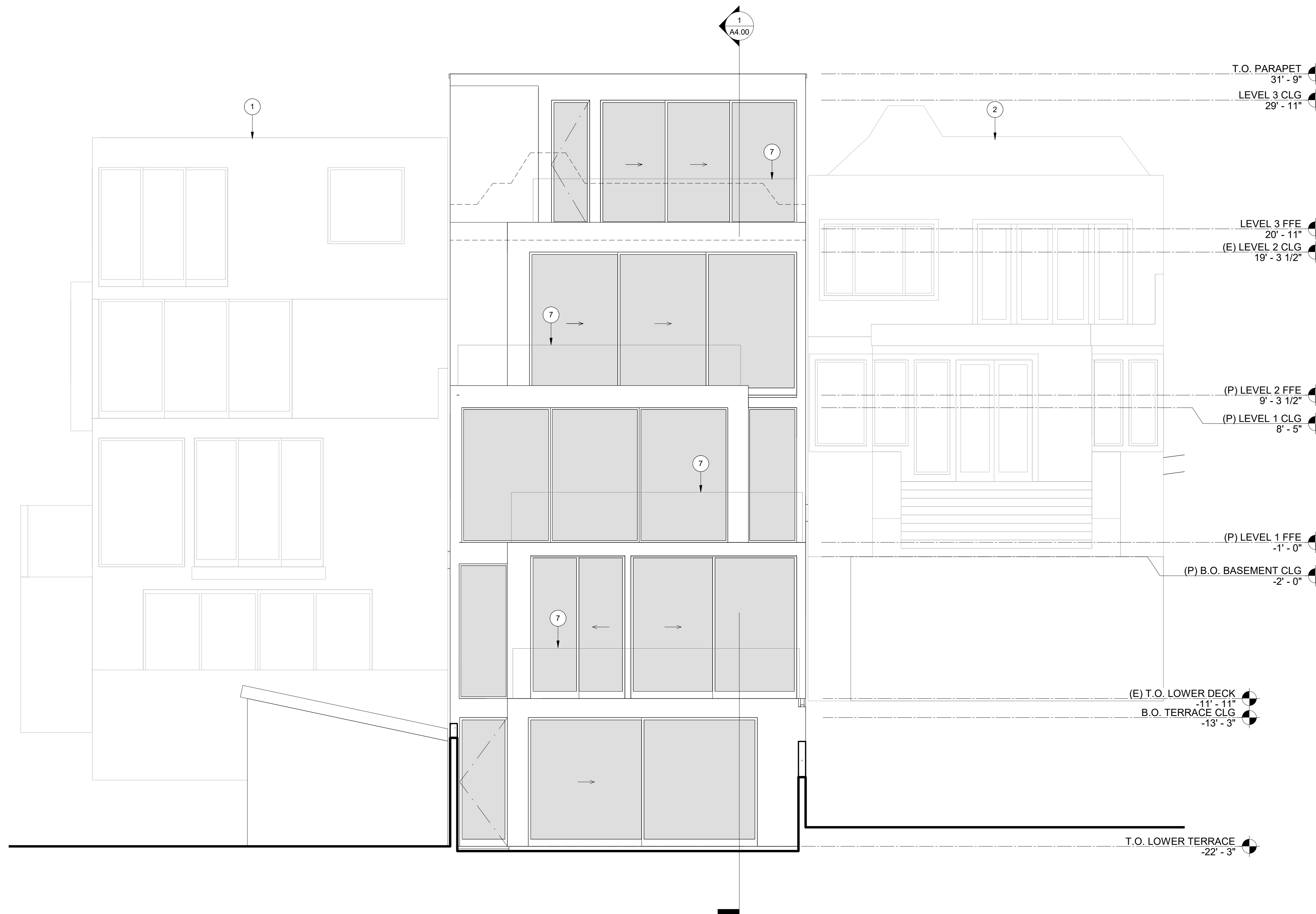
1 (P) NORTH ELEVATION 1/4" = 1'-0"
