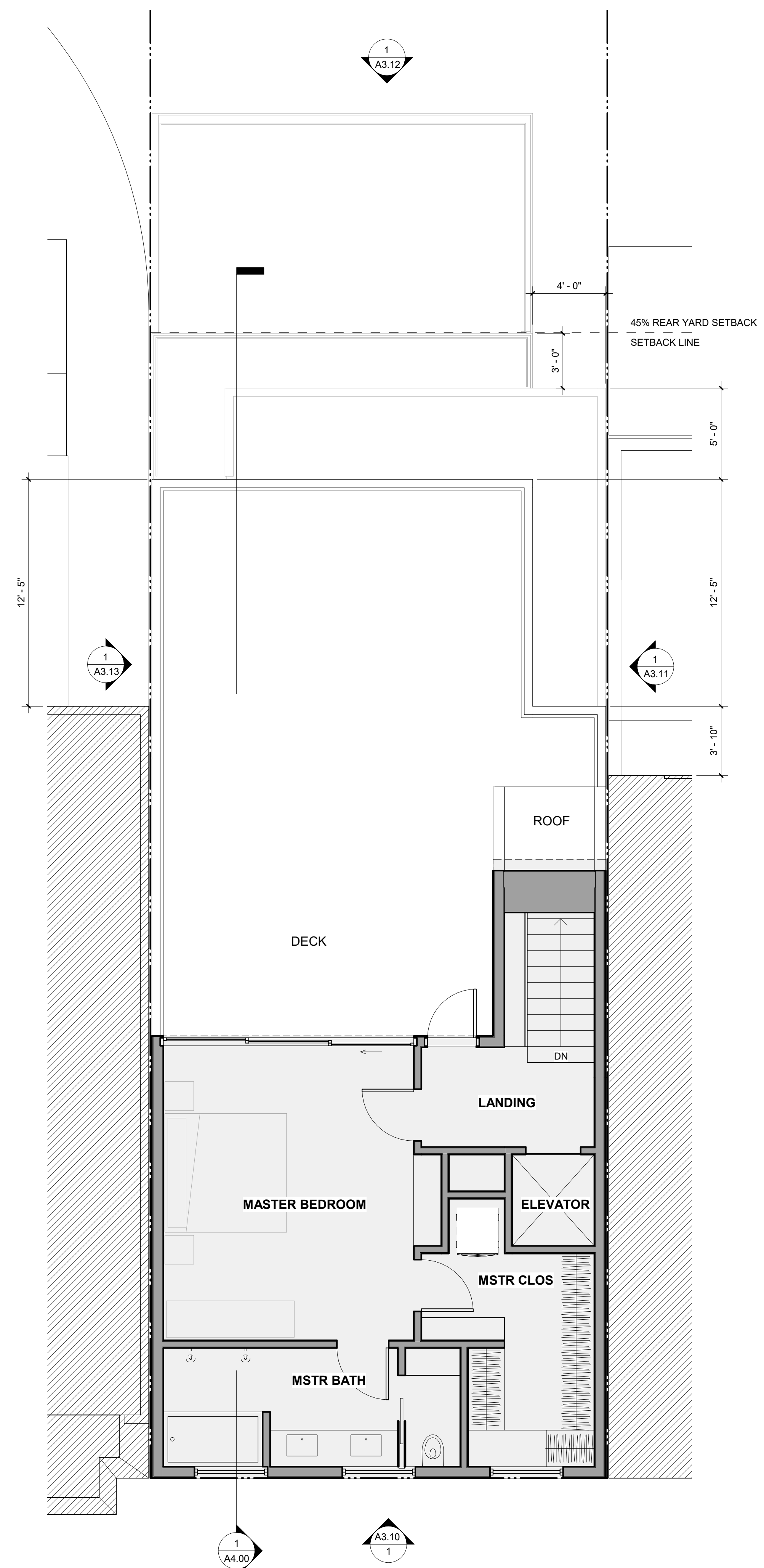
1 LEVEL 3 - PROPOSED PLAN 1/4" = 1'-0"
