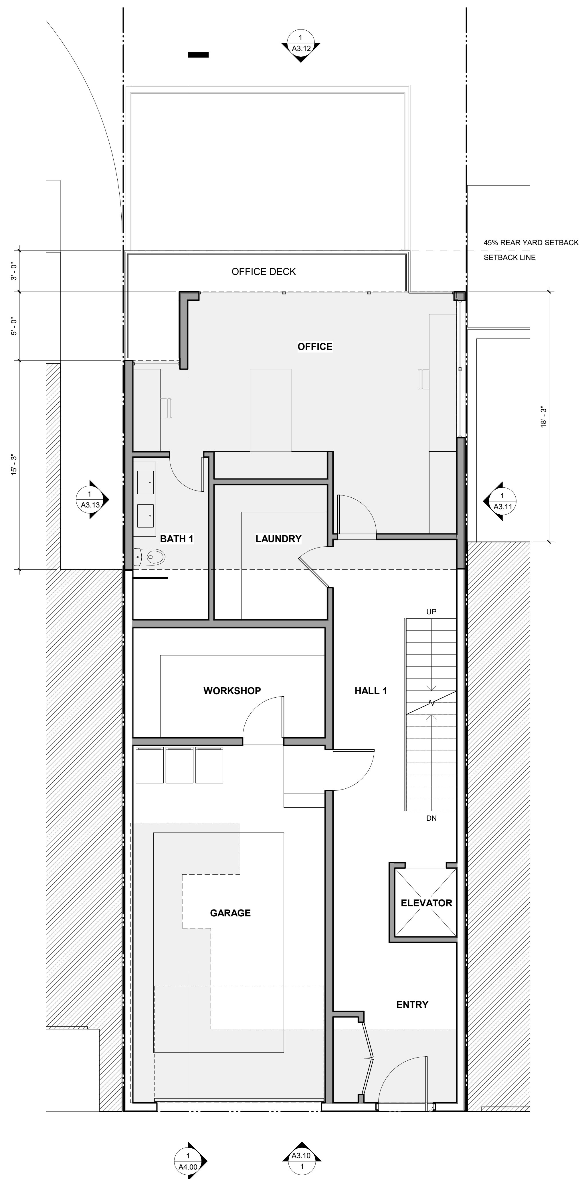
1 GROUND FLOOR - PROPOSED PLAN 1/4" = 1'-0"
