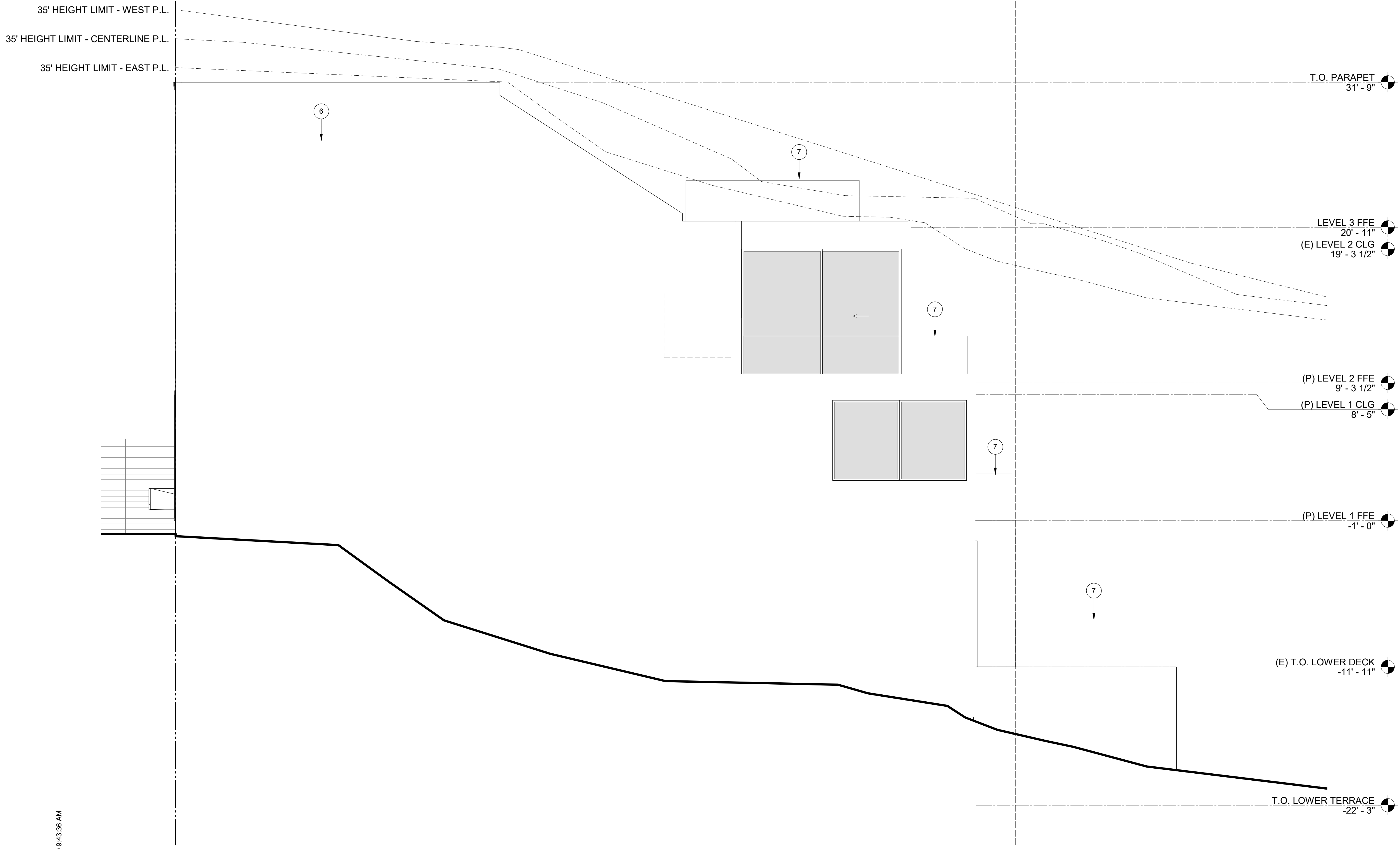
1 (P) EAST ELEVATION 1/4" = 1'-0"
