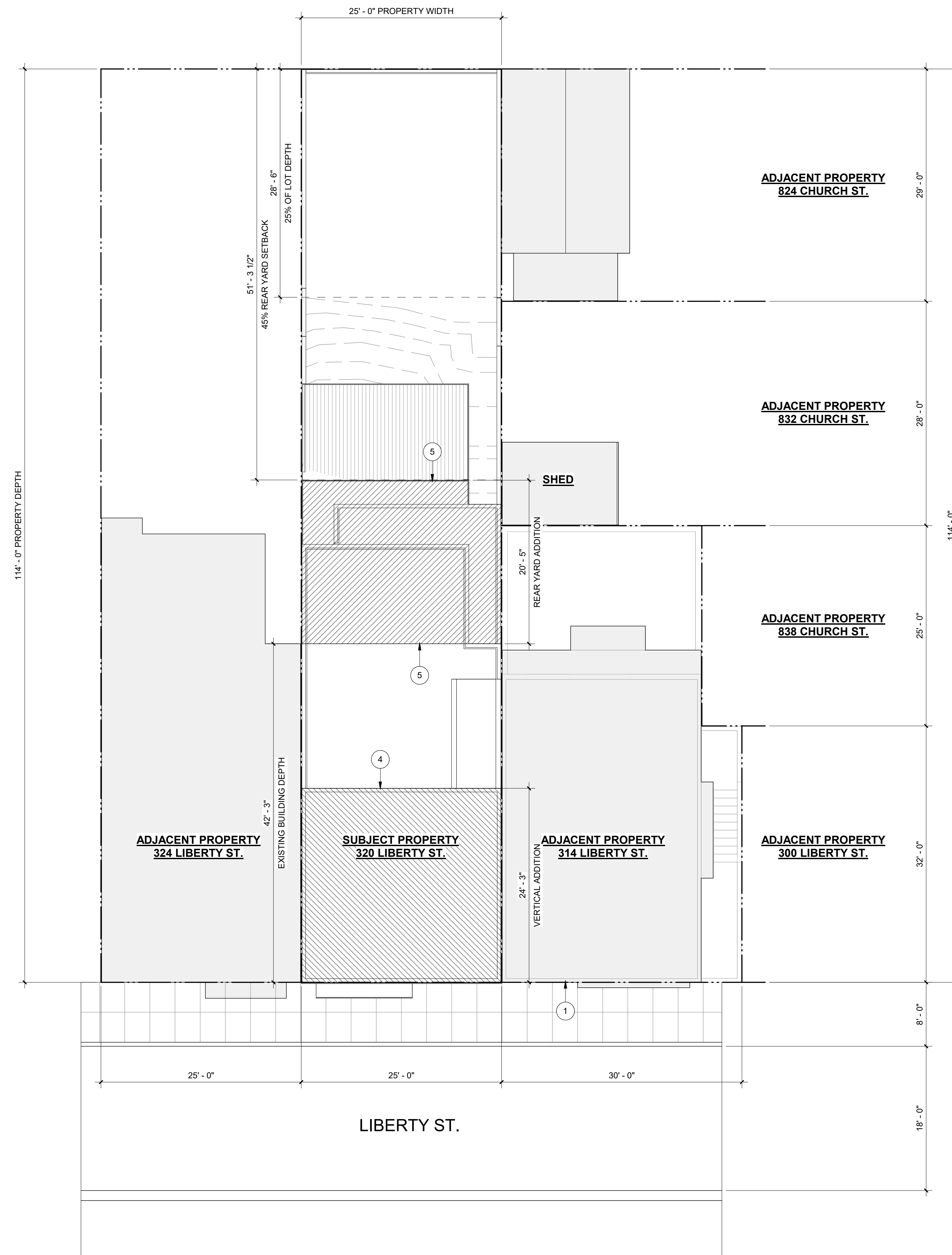
1 SITE PLAN 1/8" = 1'-0"
