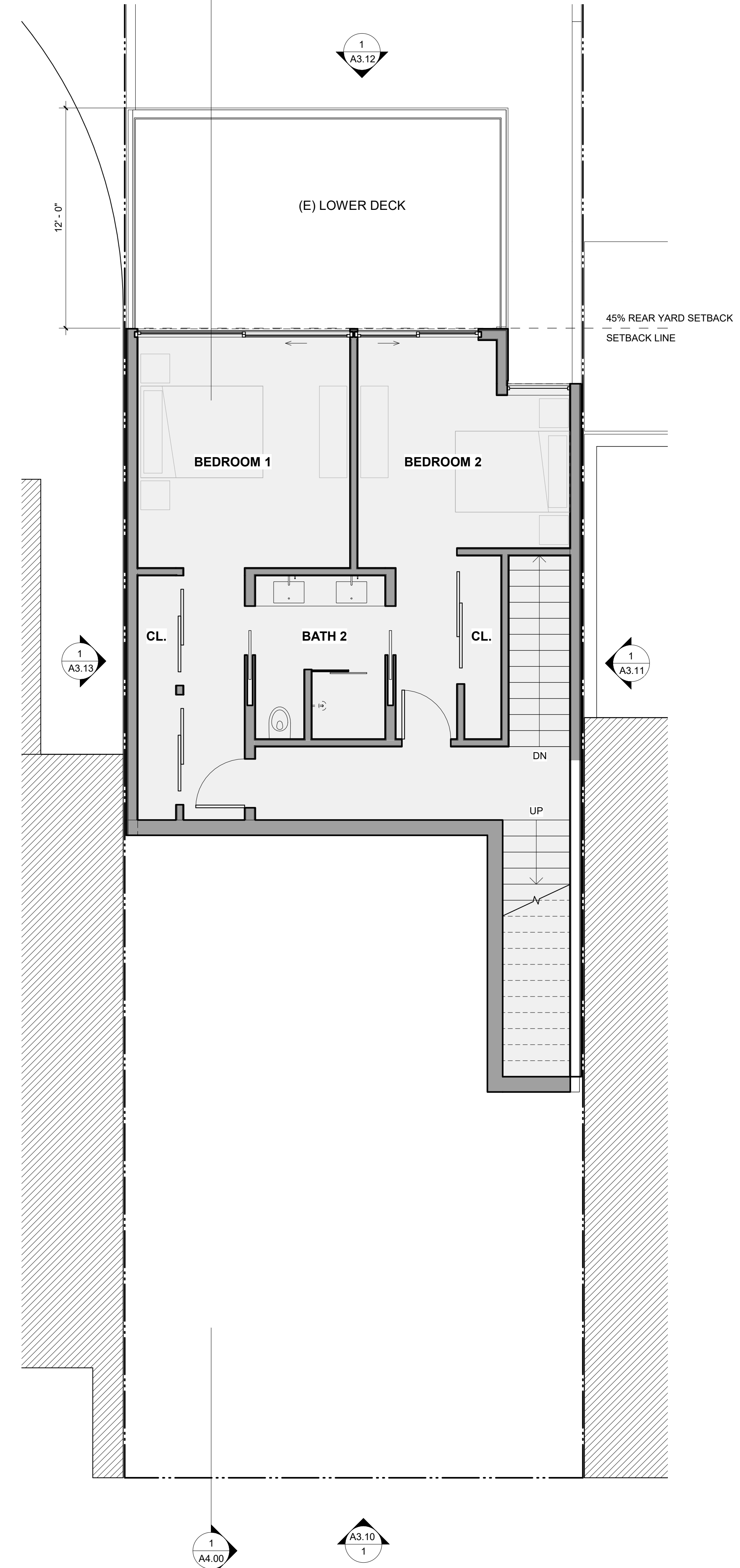
1 BASEMENT - PROPOSED PLAN 1/4" = 1'-0"
